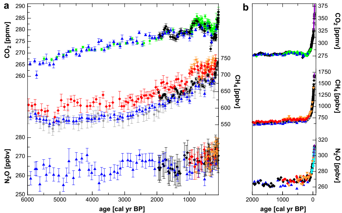
Fig. 11. Preindustrial CO 2 , CH 4 and N 2 O variations over the last 6 kyr together with their analytical reproducibility (a), and the rapid anthropogenic increase of the three greenhouse gases occurring after 1750 (b). Shown are data measured along the Greenland ice cores GRIP (red diamonds) (Blunier et al., 1995; Chappellaz et al., 1997; Flückiger et al., 1999) and Euro Core (orange triangles) (Blunier et al., 1993; Flückiger et al., 1999; Stauffer et al., 2002), together with data from the Antarctic ice cores EPICA Dome C (blue triangles) (Flückiger et al., 2002; Monnin et al., 2004), EPICA Dronning Maud Land (green circles) (Monnin et al., 2004; Siegenthaler et al., 2005), D47 (grey circles) (Chappellaz et al., 1997), and Law Dome ice and firn air samples (black diamonds) (MacFarling Meure et al., 2006). South Pole firn measurements are shown in cyan diamonds (Battle et al., 1996). Atmospheric CO 2 measurements from Mauna Loa, Hawaii ( http://cdiac.esd.ornl.gov/trends/trends.htm ) as well as CH 4 and N 2 O measurements from Cape Grim, Tasmania (Prinn et al., 2000) are shown as purple line. The offset between Greenland and Antarctic CH 4 measurements manifests the interhemispheric gradient caused by uneven distribution of the sources in the two hemispheres and the short CH 4 life time. All data are plotted on their original time scale.
