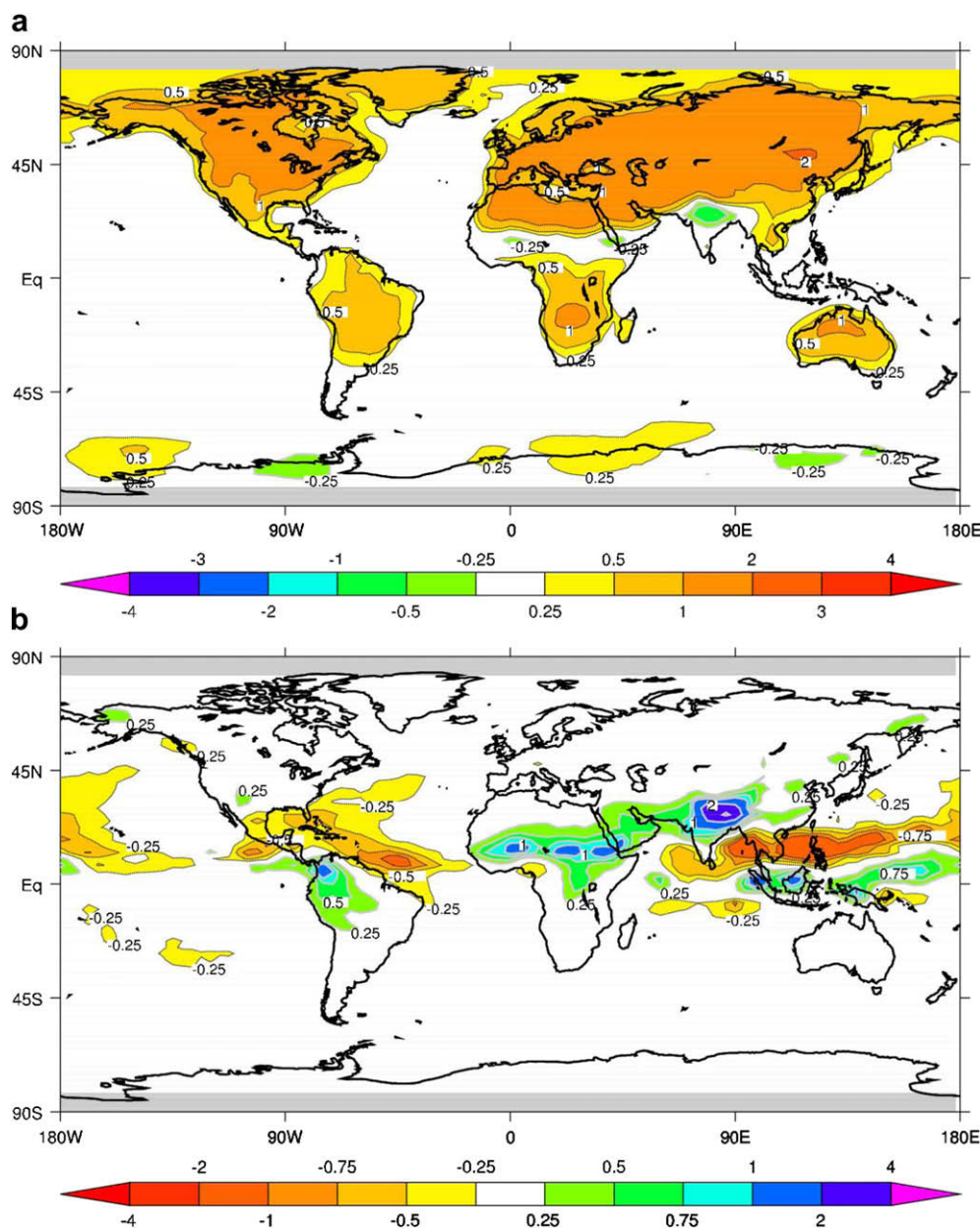
Fig. 14. Ensemble mean of PMIP2 simulations: (a) JJAS mean surface air temperature ( ^{\circ}\text{C} ) differences between Mid-Holocene and preindustrial (0 ka). (b) Same as (a) but for precipitation (mm/day). From Braconnot et al. (2007a).
