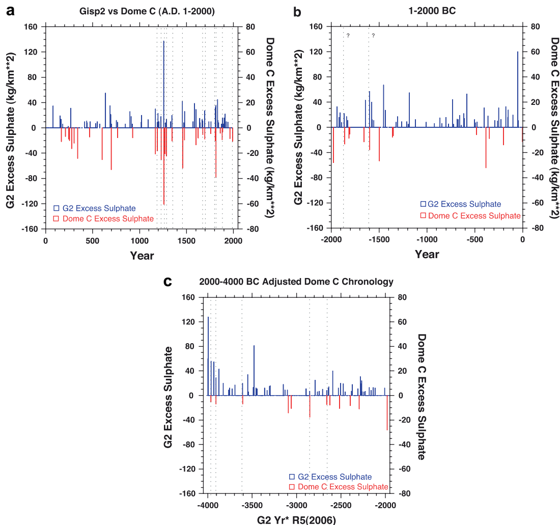
Fig. 9. Excess sulphate loadings for Dome C (Antarctica; red bars) and GISP2 ice cores (Greenland, blue bars) in kg/km 2 for the last 6000 years. The records are shown on synchronised timescales (see text for details). Vertical dashed lines indicate times of large eruptions with global influence (Crowley and Vinther, 2008).
