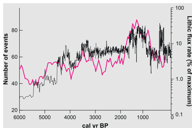
Fig. 12. Two timeseries representing the ENSO activity during the last 6000 years: (a) the black curve is based on lithic flux in marine sediments off Peru (Rein et al., 2004, 2005); (b) the pink curve represents model results by Clement et al. (2000).
