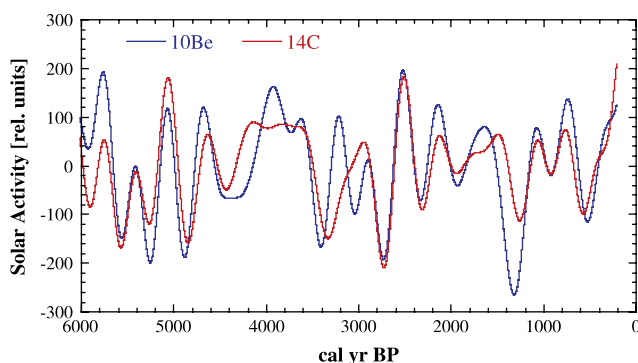
Fig. 7. Reconstructions of the solar activity based on ^{10}\text{Be} and ^{14}\text{C} . The ^{10}\text{Be} production rate was derived from ^{10}\text{Be} concentrations measured in the GRIP ice core (Vonmoos et al., 2006). The radiocarbon production rate was calculated with the Bern3D dynamic ocean carbon cycle model (Müller et al., 2006) by prescribing the tree-ring records of both hemispheres (Reimer et al., 2004; McCormack et al., 2004). Both curves were band-pass filtered with a window from 300–3000 years.
