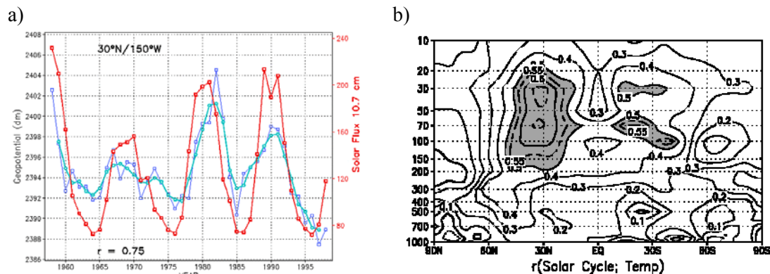
Figure 6: a) Geopotential heights at 30 hPa (blue curve) at 30N, 150W versus 10.7cm solar flux (red curve). b) Correlation between zonally averaged annual mean detrended temperatures and 10.7cm solar flux, shaded regions are for correlations > 0.5 (adapted from Labitzke and Matthes (2003)).
