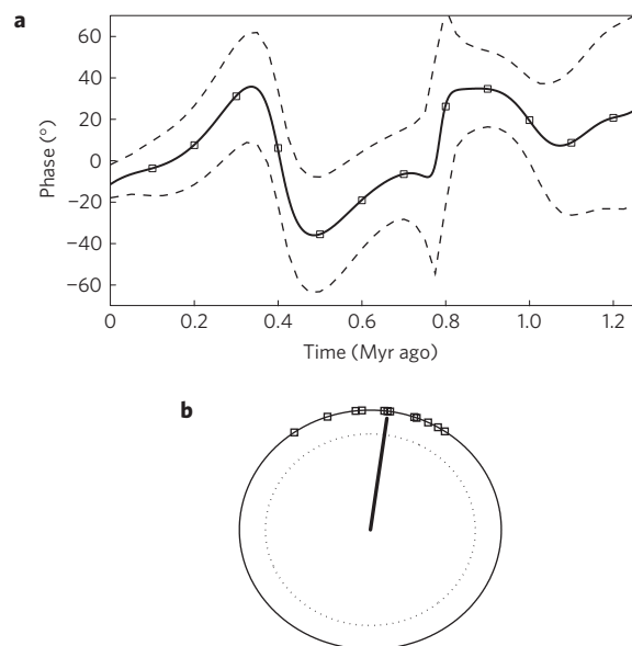
Figure 2 | 100-kyr phase. a, Phase lag of untuned \delta^{18}\text{O} relative to eccentricity calculated by cross-wavelet analysis. The dashed lines are 1\sigma error bars based on age-model uncertainty (see Supplementary Information). The squares mark where the phase is sampled every 100 kyr for calculation of the Rayleigh statistic. b, Phase wheel representation of the 100-kyr phase (squares) of untuned \delta^{18}\text{O} from 1.2 to 0 Myr ago. The vector length is the Rayleigh R value (0.94) and its angle shows the mean phase lag ( 7.7^\circ , 1.2 kyr). The dotted circle marks the 5% significance level ( R = 0.80 ) for eccentricity pacing.
