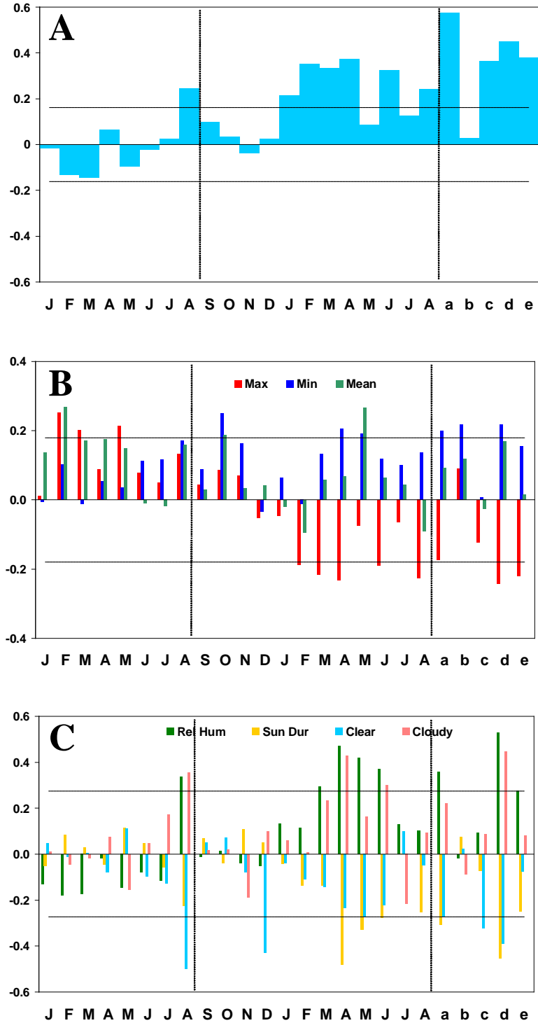
Fig. 5 Climate response plots for the Lamington National Park site with Brisbane meteorological data: Monthly coefficients of correlation for precipitation (A), maximum, minimum and mean temperatures (B) and relative humidity, sunshine duration and number of clear and cloudy days (C). The climate response plots are subdivided into three parts by vertical hatched lines. The left half of the diagram covers the period January to August before the current season, the middle part stands for this season (September to August) and the small letters a to e stand for the annual value and the averages for the periods for September to November, December to February, March to May and June to August of the current season, respectively. In each diagram the 95 % confidence intervals are indicated by the horizontal hatched lines with different levels due to available time series lengths (Source: Australian Bureau of Meteorology Canberra 2002)
