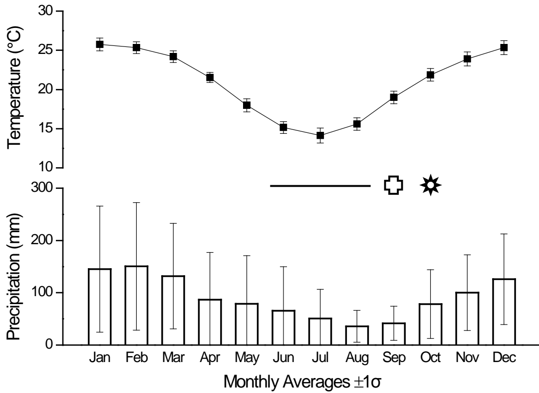
Fig. 2 Climate diagram derived from long-term averages for Brisbane meteorological station, (Source: Australian Bureau of Meteorology, Canberra 2002); the phenology of Toona ciliata is marked by a line (leafless period, June to August), cross (leaf flushing, September) and asterisk (flowering, October)
