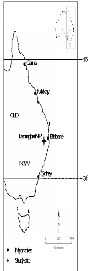
Fig. 1 Location of the study site Lamington National Park indicated by the asterisk; the old-growth montane subtropical rainforest is located in southeast Queensland 600 to 900m asl ( 28^{\circ} 15' S , 153^{\circ} 08' E )
