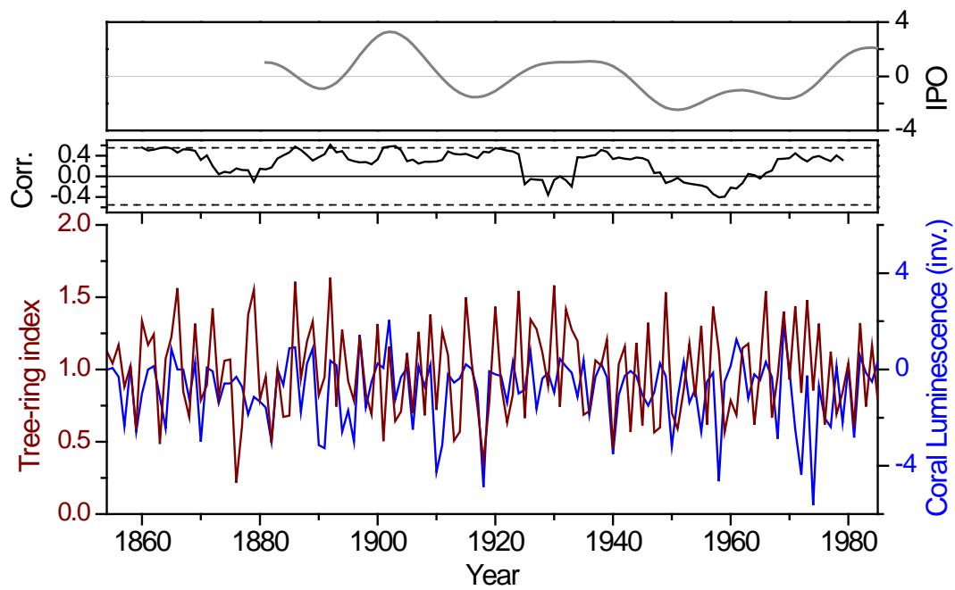
Fig. 9 Lamington National Park tree-ring site chronology (brown) in comparison to the coral luminescence master chronology (Hendy et al. 2003) (blue); Pearson's correlation (Corr.) calculated in moving windows of 13 years (95 % confidence levels are indicated); for comparison printed on top, the Interdecadal Pacific Oscillation Index (Folland et al. 1999; Power et al. 1999, kindly provided by the UK Met Office) (grey)
