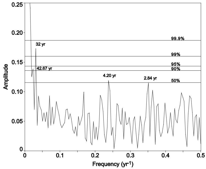
Fig. 8 Spectral analysis of the Lamington National Park tree-ring width index for the period 1854-2000 shows significant peaks at approximately 42 and 32 years. 50, 90, 95, 99 and 99.9 % confidence levels are indicated
