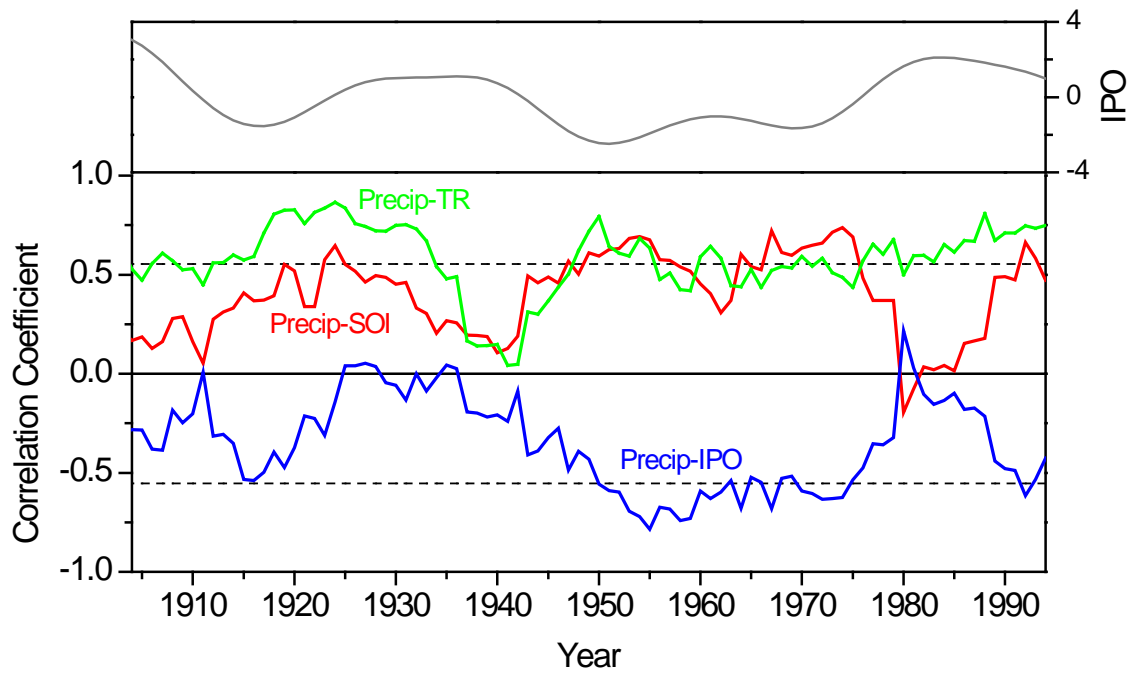
Fig. 10 Coefficients of correlation between Brisbane precipitation and Lamington National Park tree-ring chronology (green), Southern Oscillation Index (red) and Interdecadal Pacific Oscillation (blue) in moving windows of 13 years (95 % confidence levels are indicated); for comparison printed on top, the Interdecadal Pacific Oscillation Index (Folland et al. 1999; Power et al. 1999, kindly provided by the UK Met Office) (grey)
