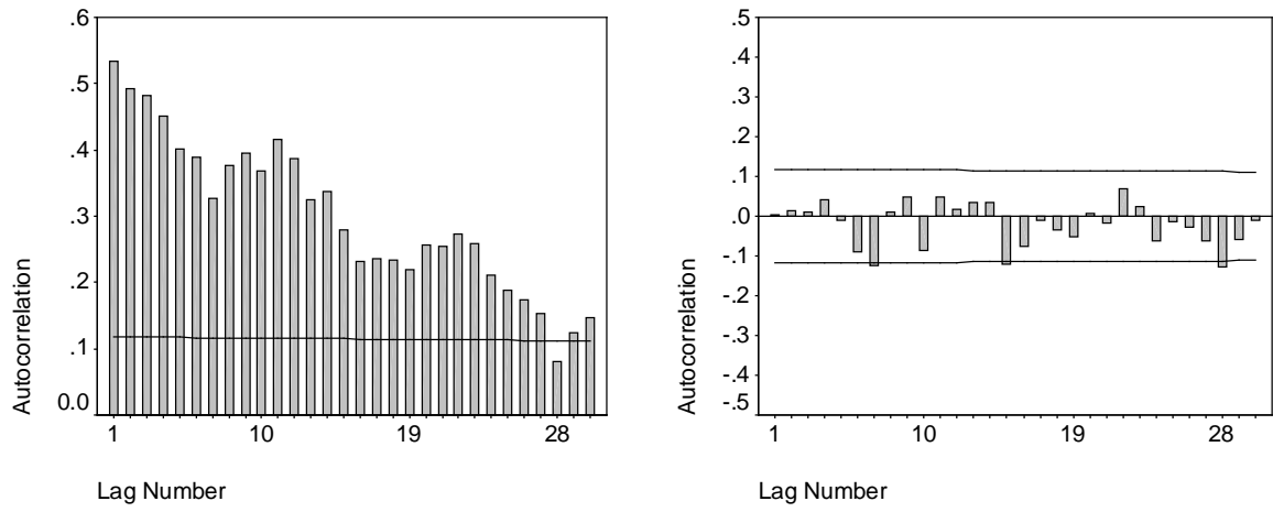
Fig. 3 Autocorrelation (lags 1 to 30) for the raw (left) and detrended (right) tree-ring values from the Lamington National Park site
