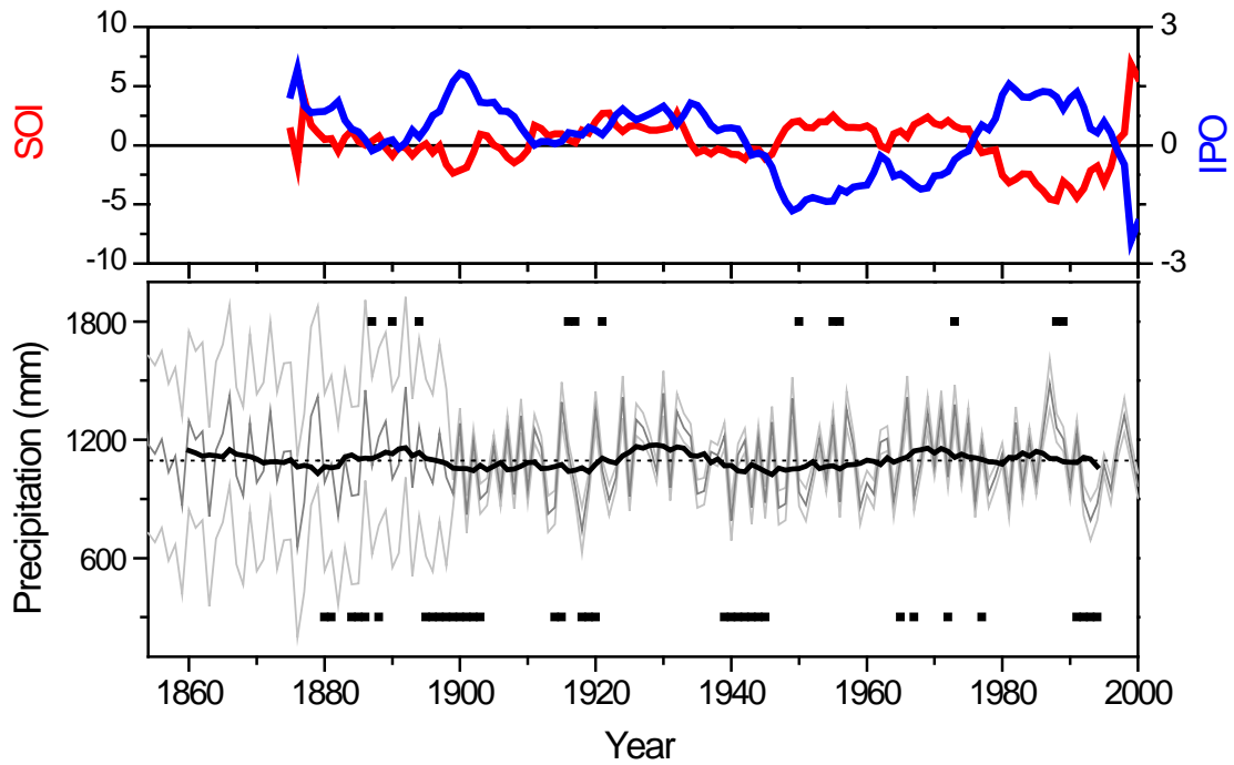
Fig. 7 Reconstructed annual precipitation for Lamington National Park (dark grey line) with 13-year running mean (black line) and 95% confidence intervals (light grey lines) in comparison to major drought (lower markings) and flooding events (upper markings) (Whetton, 1997) and 13-year running means of SOI (Australian Bureau of Meteorology Canberra 2002) (red) and IPO (Folland et al. 1999; Power et al. 1999, kindly provided by the UK Met Office) (blue)
