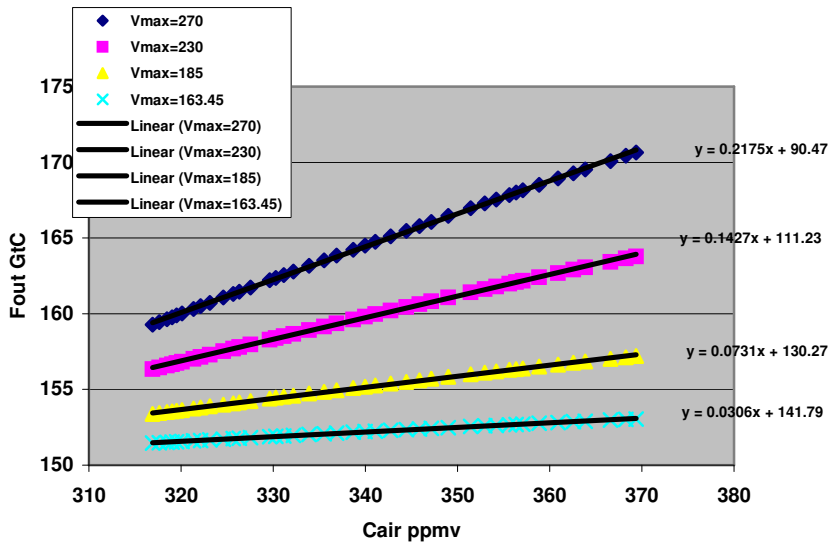
Figure 10. Hypothetical curves for flow into the sinks with model M: F_{out} = V_{max} * C_{air} / (K_m + C_{air}) with assumed F_{na} > 0 The regression lines indicate the correspondence of the Michaelis Menten equation with linear equations.
