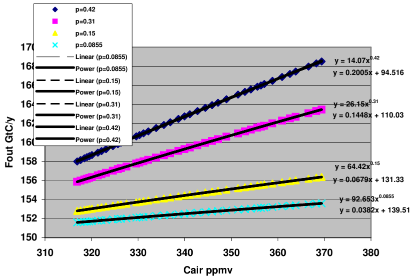
Figure 9. Hypothetical curves for flow into the sinks with model P: F_{out} = k \cdot C_{air}^p with assumed F_{na} > 0 . The regression lines indicate the correspondence of the power equation with linear equations.
