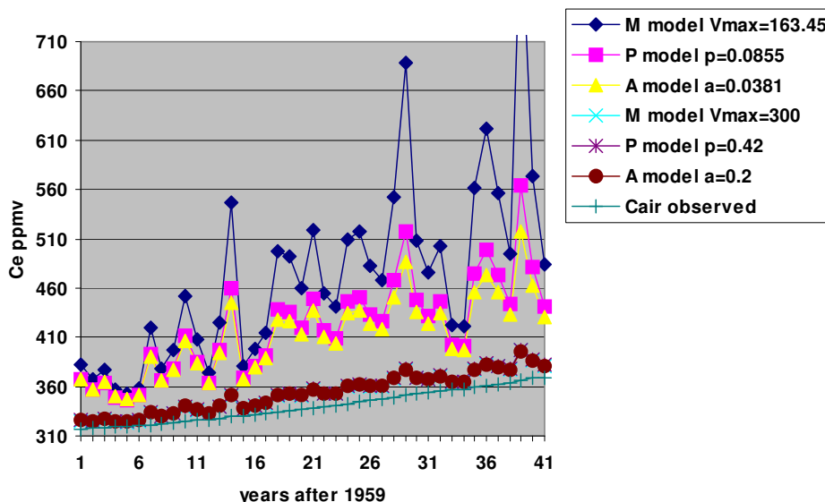
Figure 12. The calculated equilibrium state in each year for the three models with F_{na} = 0 and assumed values F_{na} > 0 .
