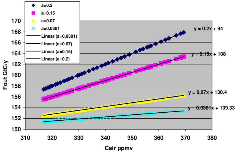
Figure 8. Hypothetical curves for flow into the sinks with model A: F_{out} = aC_{air} + b with assumed F_{na} > 0
