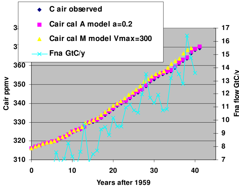
Figure 11. The match of calculated rise of CO 2 in the atmosphere with model A and model M when a high natural flux (F na ) is involved. The F na flow (right Y axis) is calculated from the equation: F_{na} = 0.2 * C_{air} + 94 - (F_o + F_{em} - F_a)
