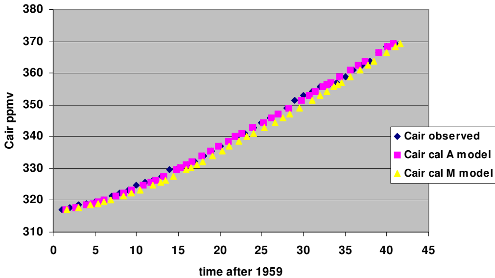
Figure 6. Comparison of the observed \text{CO}_2 in the atmosphere with the predictions of the M and A models.
