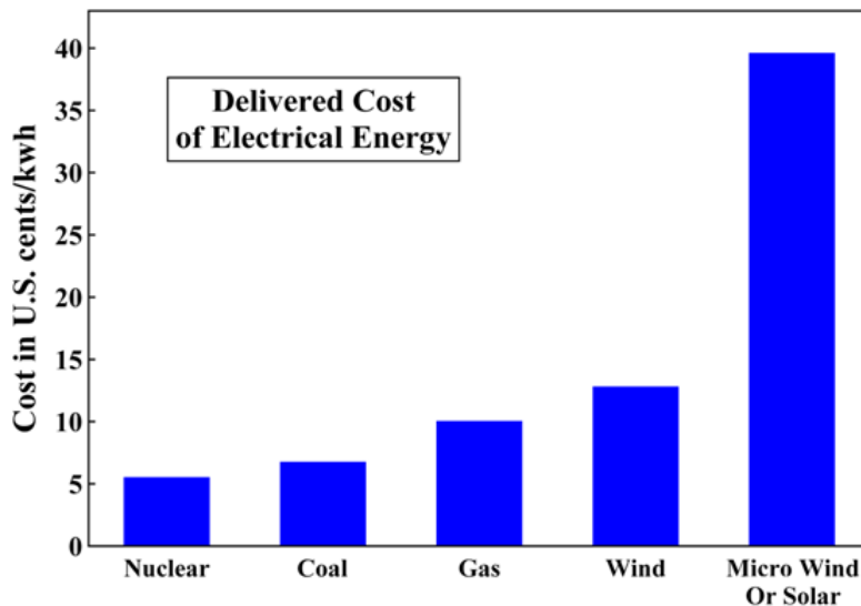
Figure 26: Delivered cost per kilowatt hour of electrical energy in Great Britain in 2006, without CO2 controls (126). These estimates include all capital and operational expenses for a period of 50 years. Micro wind or solar are units installed for individual homes.
