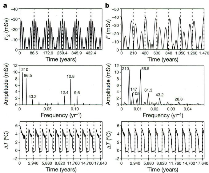
Figure 4 | Model response for non-sinusoidal forcing profiles. a , Roughly 86.5-year Gleissberg cycle implemented as amplitude modulation of a \sim 11 -year cycle (representing the Schwabe solar cycle). Top panel: combined Gleissberg/Schwabe forcing component F_2 = -A_2 |\cos(\omega_2 t/2)| |\cos(\omega_3 t/2)| . The chosen forcing parameters are A_2 = 30 mSv, \omega_2 = 2\pi/T_2 ( T_2 = 1,470/17 years \approx 86.5 years), \omega_3 = 2\pi/T_3 ( T_3 = 1,470/136 years \approx 10.8 years). |\cos(\omega t/2)| is used because |\cos(\pi t/T)| has a period of T . The 210-year DeVries component F_1 is considered as an additional cosine cycle, identical to that in Fig. 1a: F_1 = -A_1 \cos(\omega_1 t) with A_1 = 10 mSv and \omega_1 = 2\pi/T_1 ( T_1 = 1,470/7 years = 210 years). Note: here, the freshwater axis is inverted compared with that in Fig. 1. The total forcing is the sum of both components plus an offset K = -5 mSv. Middle panel: Fourier spectrum of F_1 + F_2 . The spectrum is discrete because the forcing is periodic. Numbers above peaks are years. Bottom panel: model response. b , Gleissberg cycle modulated by the DeVries cycle. Top panel: combined DeVries/Gleissberg forcing component F = -A_1 |\cos(\omega_1 t/2)| |\cos(\omega_2 t/2)| . The chosen forcing parameters are A_1 = 40 mSv, \omega_1 = 2\pi/T_1 ( T_1 = 1,470/7 years = 210 years), \omega_2 = 2\pi/T_2 ( T_2 = 1,470/17 years \approx 86.5 years). The total forcing is given by F plus an offset K = 5 mSv. Middle panel: Fourier spectrum of F . Bottom panel: model response.
