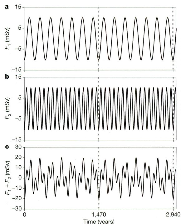
Figure 1 | Applied freshwater forcing in the simulation. a, b , To represent the DeVries and Gleissberg solar cycles we consider two sinusoidal components: DeVries component F_1 with period T_1 = 210 years ( a ) and Gleissberg component F_2 with period T_2 \approx 86.5 years ( b ). c , Total forcing ( F_1 + F_2 ). The dashed lines indicate the period of 1,470 years in the forcing. In the figure, the amplitudes A_1 and A_2 are chosen to be 10 mSv and the phases \varphi_1 and \varphi_2 to be 0. The additional offset K is not shown here.
