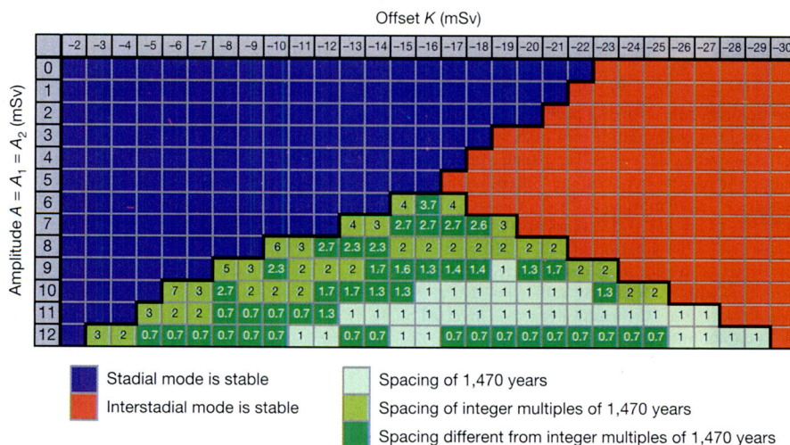
Figure 3 | Schematic response of the model for different amplitudes A (with A = A_1 = A_2 ) and offsets K in the forcing. Upper left area (blue): ‘cold’ regime (stadial mode is stable). Upper right area (red): ‘warm’ regime (interstadial mode is stable). Lower area (green): ‘Dansgaard–Oeschger’
