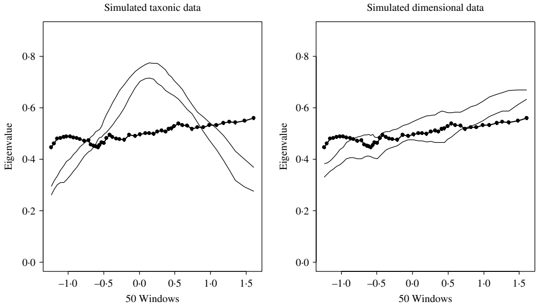
FIG. 2. Average MAXEIG (MAXimum EIGenvalue) curves for the research data, simulated taxonomic data, and simulated dimensional data for the four SCID-II antisocial personality disorder (ASPD) factor scores. For each curve, the data were sorted along the x axis by the scores on the input indicator and then grouped into 50 subsamples using overlapping windows (0.90 overlap). The graphs for the simulated taxonomic and dimensional data were produced by generating 10 datasets for each latent structure. The dark line represents the actual data and the lighter lines represent one standard deviation above and below the average for each simulated dataset.
